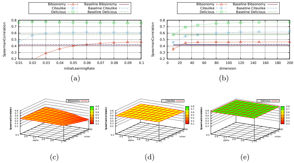
Figure 2: Evaluation results for embeddings generated by GloVe on the MEN dataset. The initial learning rate only influences the smaller tagging datasets, while Delicious profits most from increasing dimension. BibSonomy is influenced by a high cutoff x_{max} the most.
