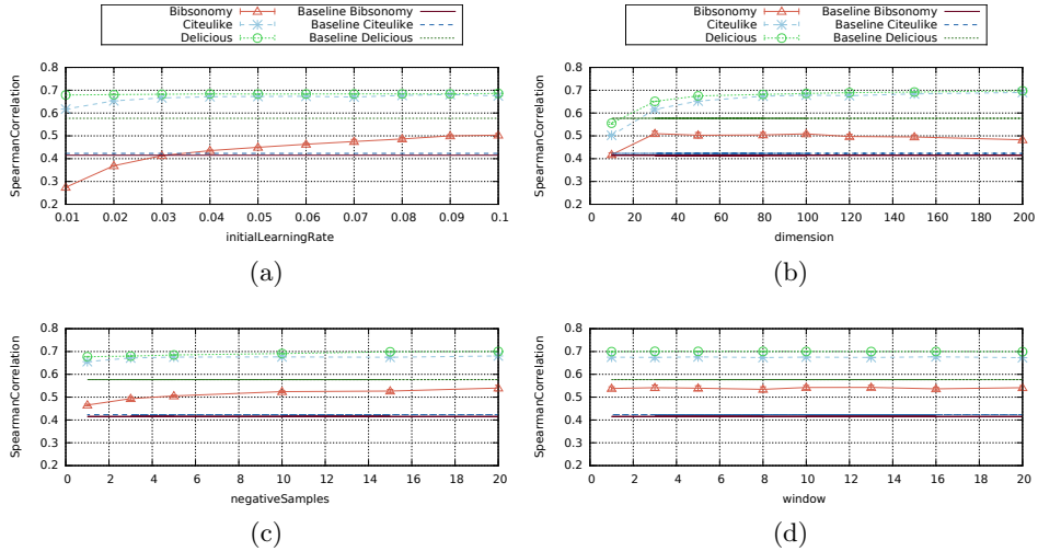
Figure 1: Evaluation results for embeddings generated by Word2Vec on MEN. For CiteULike and BibSonomy, tuning the learning rate notably improves results. The embedding dimension seems to be the best for all tagging dataset at 100; afterwards the quality of BibSonomy embeddings decreases again. As reported by [24], a number of around 10 negative samples seems sufficient for small datasets such as BibSonomy, while a lesser number of samples fits for bigger datasets.
