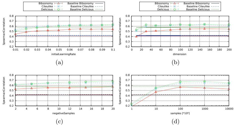
Figure 3: Evaluation results for embeddings generated by LINE on the MEN dataset. While the initial learning rate, the embedding dimension and the amount of samples per step exert a notable influence on the evaluation result, increasing the number of negative samples per edge only slightly improves results.
